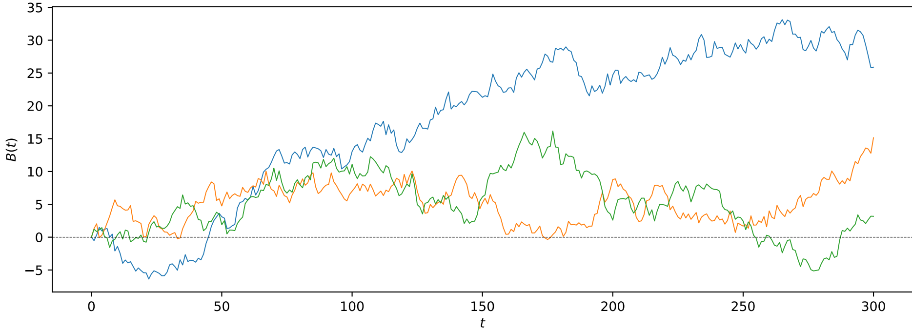
Standard Brownian Motion B(t) , 3 realizations
